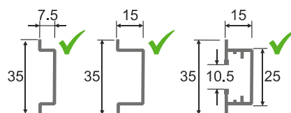
Fig. 5-4: Mounting rails
