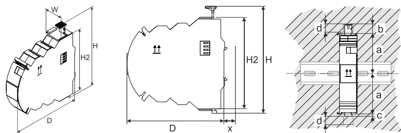
Fig. 4-9: Dimensions
