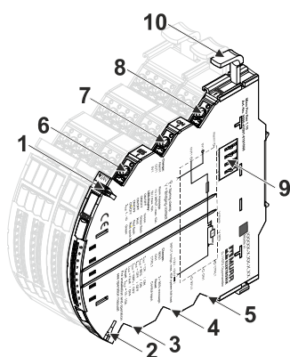
Fig. 6-3: Installation overview
