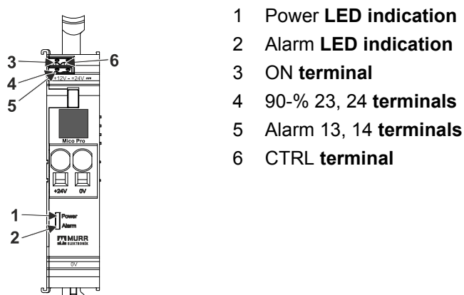
Fig. 7-1: Operation overview
