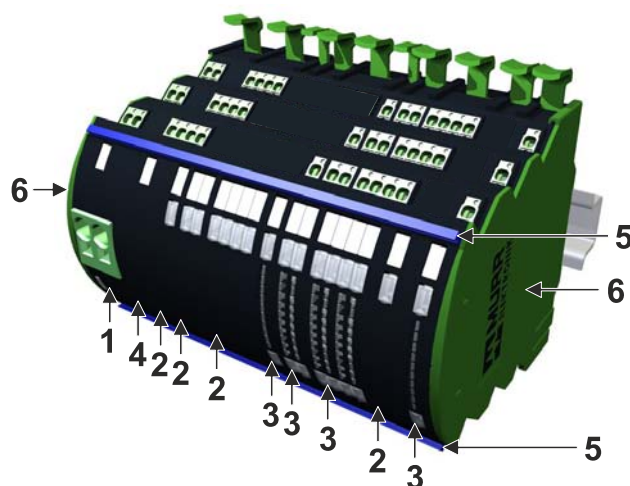
Fig. 3-1: Example of assembly
